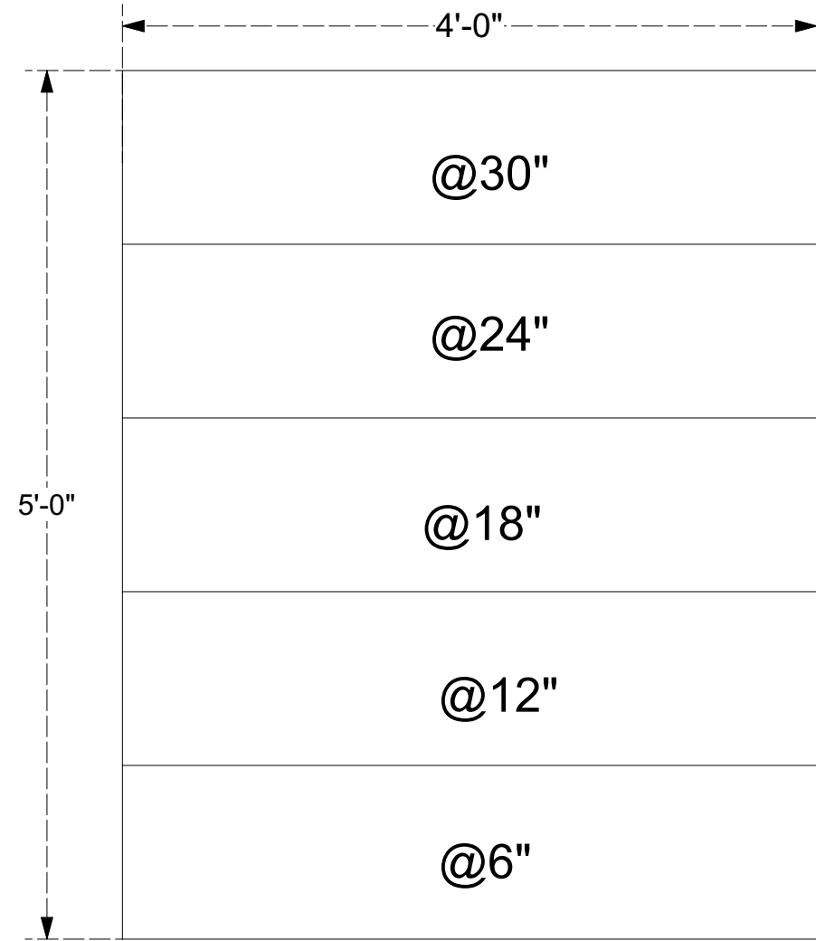
Top View
